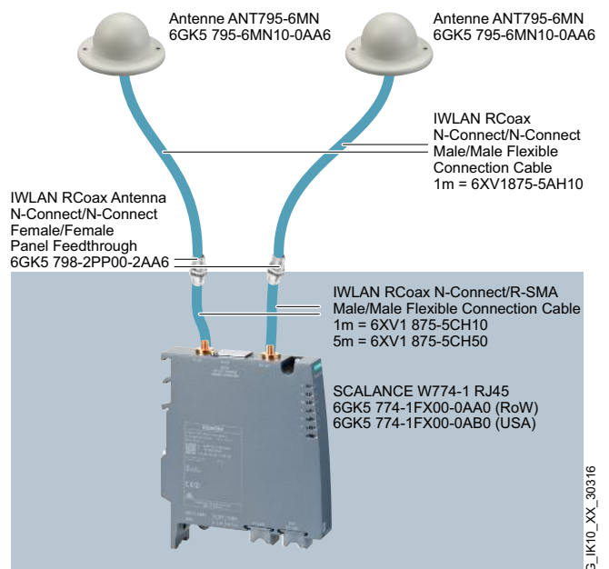
SCALANCE W774-1RJ45 with detached antenna (lateral)
